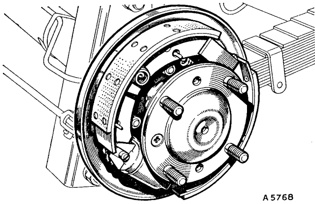
Fig. M.10 The rear brake assembly
